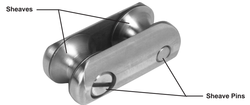
Figure 1. Rope to Rope/Grip Clevis
